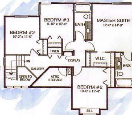
SECOND FLOOR PLAN 945 SQ. FT. (87.8 M 2 )
