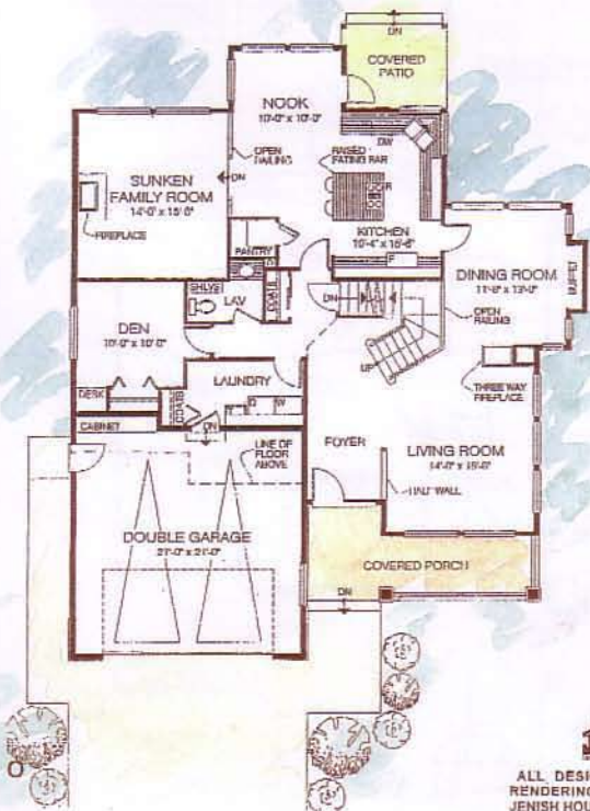
MAIN FLOOR PLAN 1572 SQ. FT. (146.0 M 2 )
